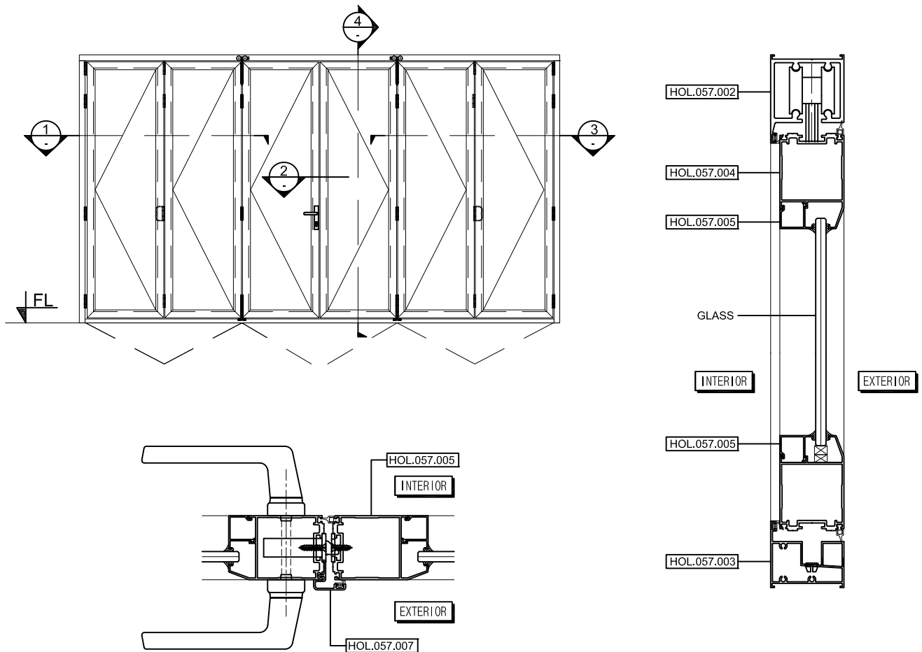
2 Horizontal Section Detail SCALE : NONE
